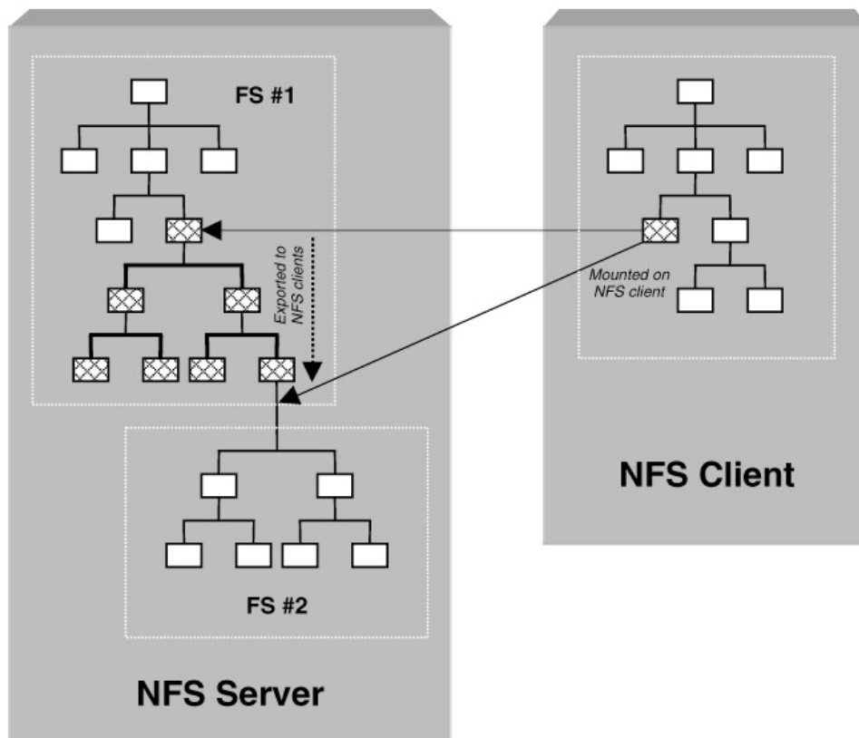
Figure 18.1: Exporting NFS.
