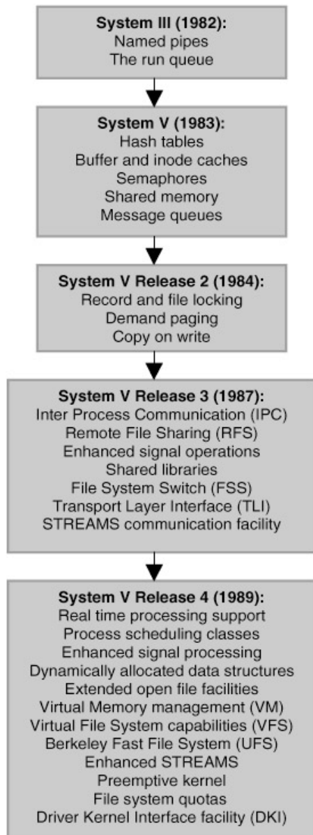
Figure 1.2: The development of ATT UNIX.
