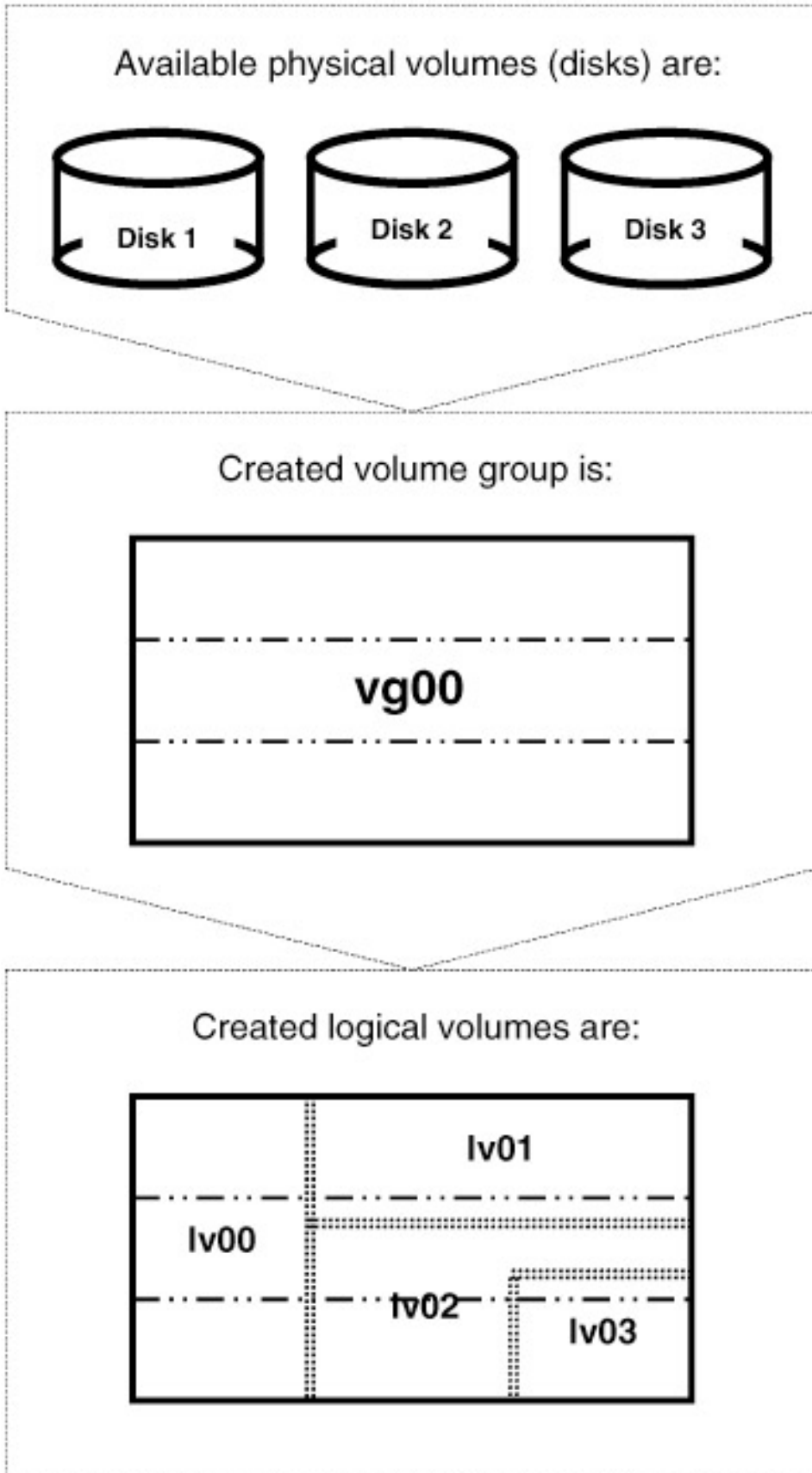
Figure 6.6: AIX data storage organization. The LVM provides the necessary physical-to-logical mapping (and vice versa) and handles filesystems. Although very complex mapping and processing is going on, everything is hidden from the users. They simply use the available storage units.
