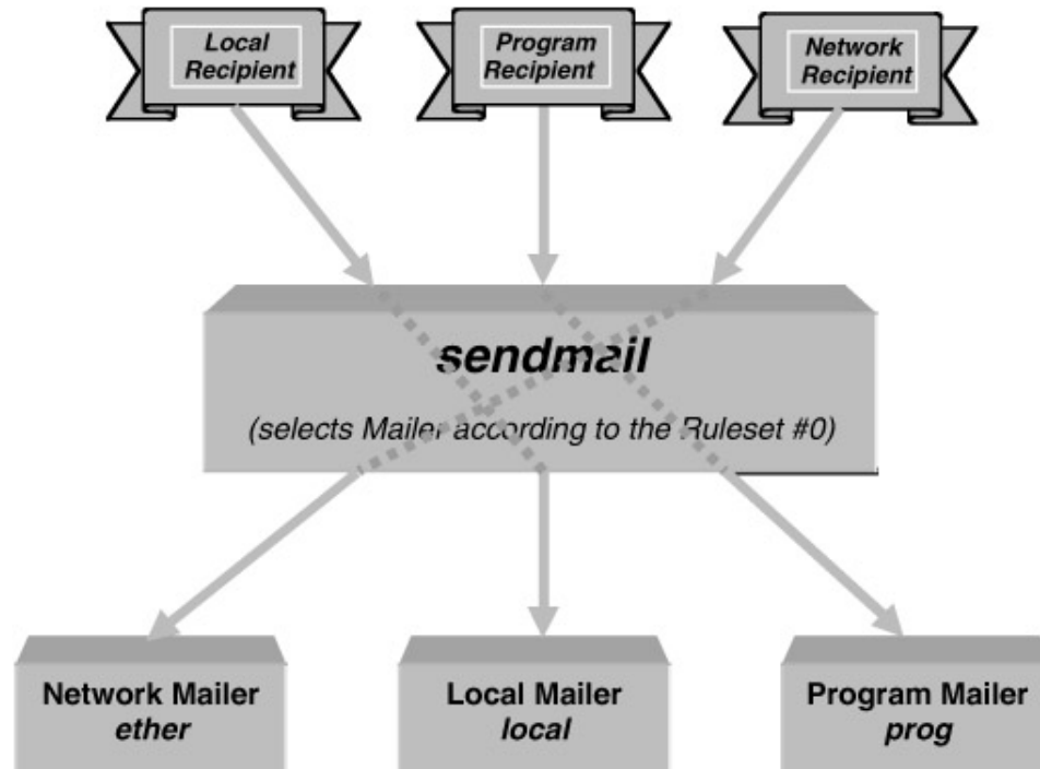
Figure 20.3: Sendmail vs. mailers relations.
