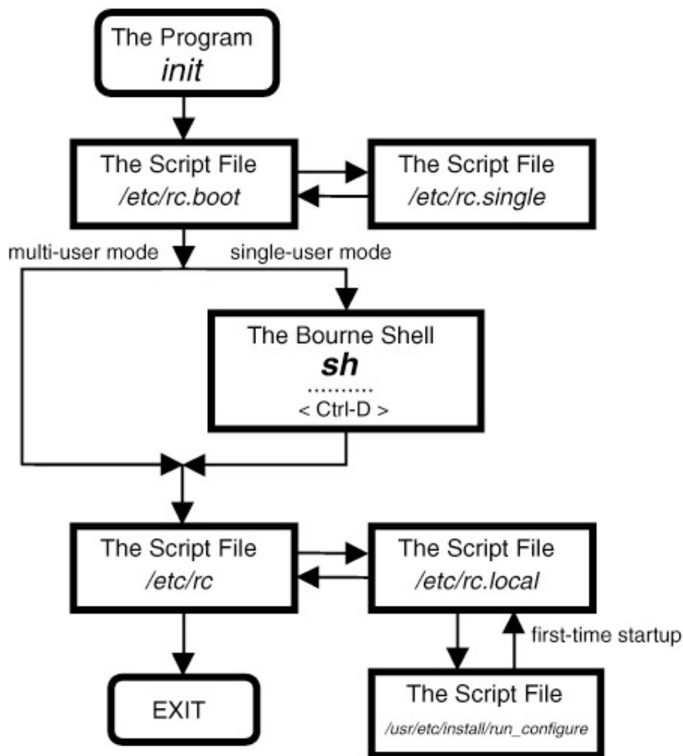
Figure 4.3: The execution sequence of SunOS initialization scripts.
