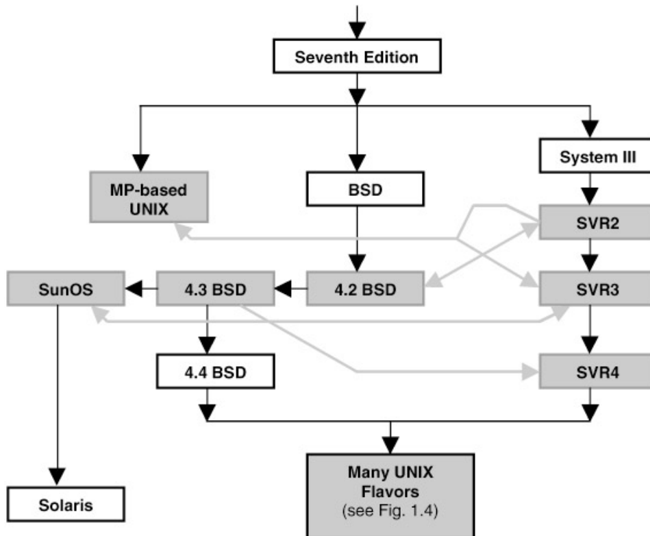
Figure 1.3: UNIX genealogy.
