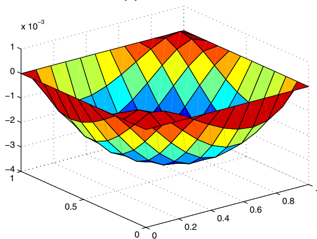
Sol app – Sol exacte
