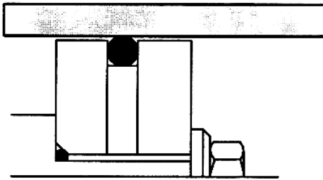
Joint torique
