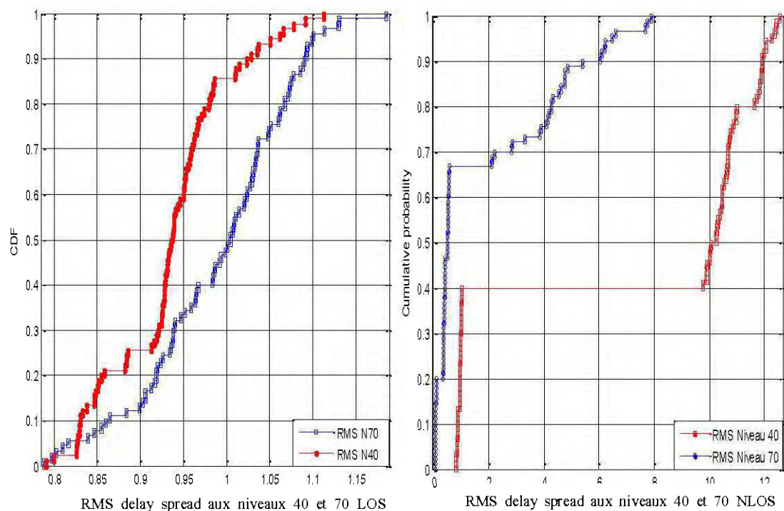
Figure 5-16: Courbes comparatives du RMS delay spread aux niveaux 40m et 70m.
