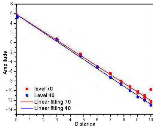
Fig. 4 Path loss vs. distance (LOS)
