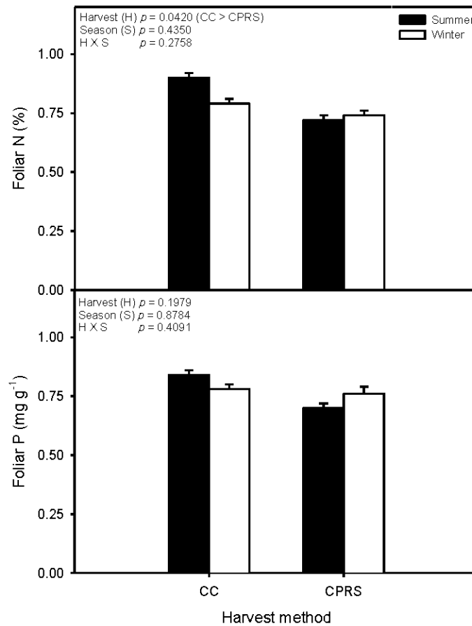
Figure 2.3. Black spruce foliar N ( \% \pm 1 S.E.) and P ( \text{mg g}^{-1} \pm 1 S.E.) according to harvest method and season. CC = clearcut, CPRS = cut with protection of regeneration and soils.
