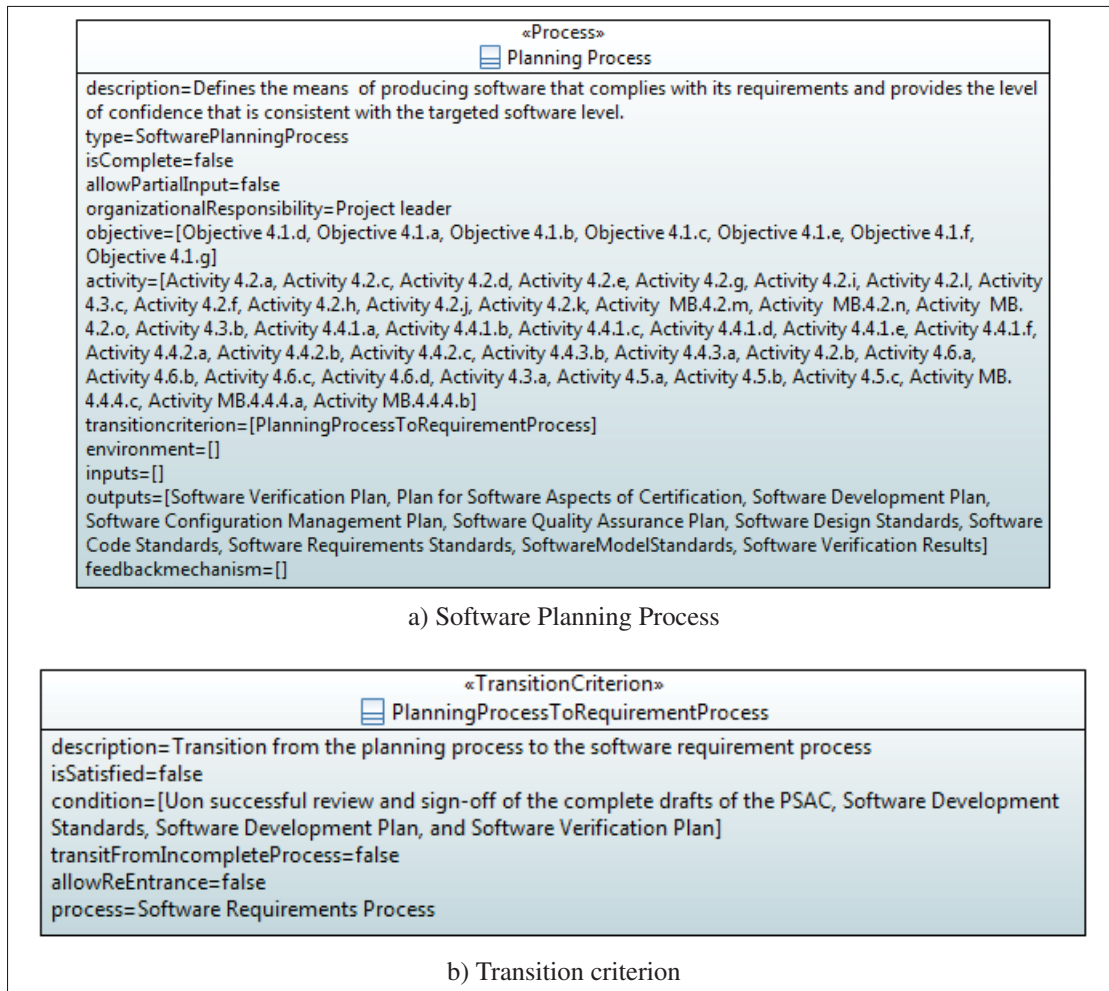
Figure 5.11 The software planning process and its apportioned transition criterion.
