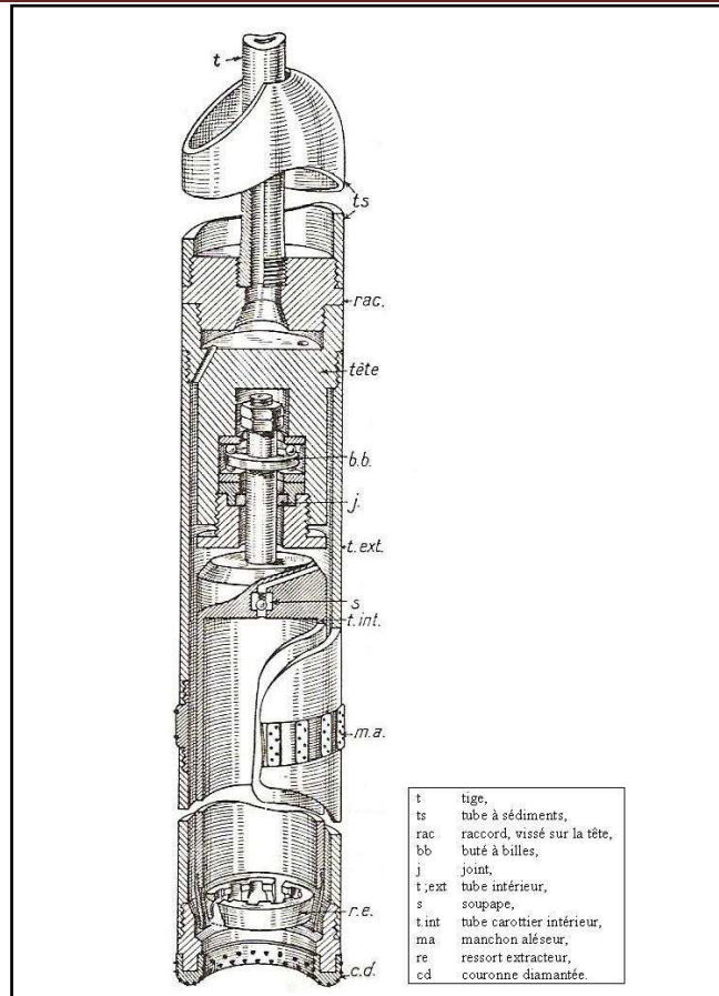
Figure 8: Double carottier
