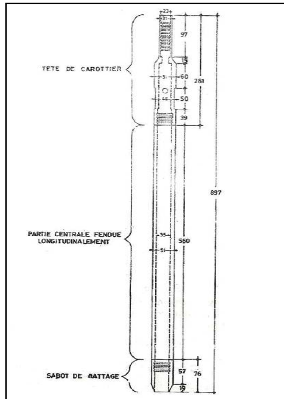
Figure 7: Carottier S.P.T.
