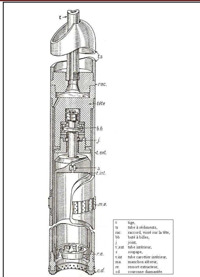
Figure 8: Double carottier
