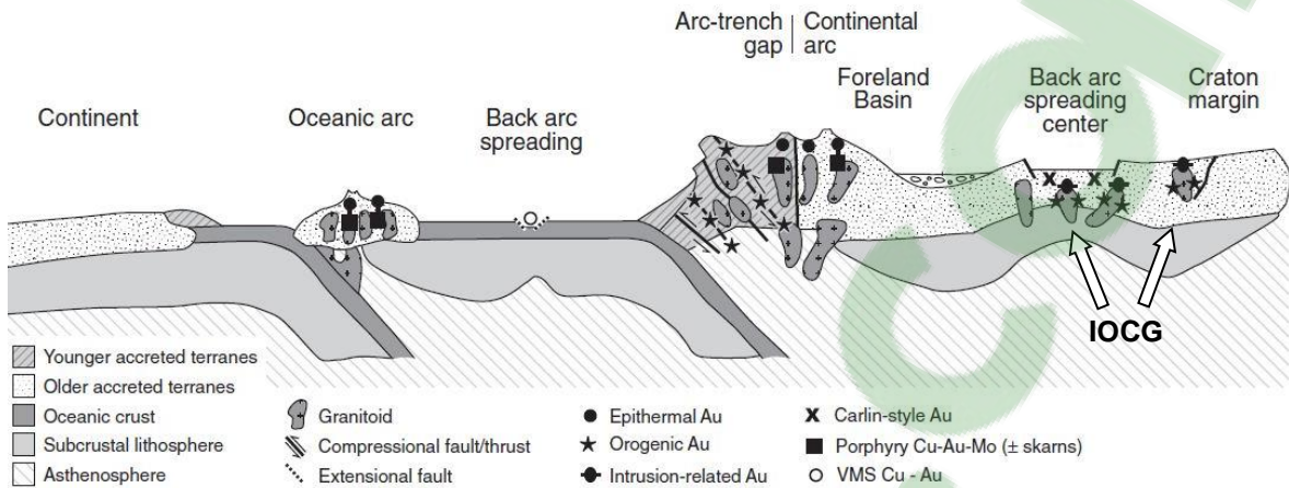
FIG. 2. Schematic diagram showing the tectonic setting of various gold deposit types. Orogenic gold deposits develop in the forearc region of a convergent continental margin over a wide range of crustal depths and may also develop in deformed back-arc sedimentary sequences seaward of the craton margin. Reduced intrusion-related gold deposits form inland of accreted terranes along shelf sequences of a craton margin. After Groves et al. (2005).
