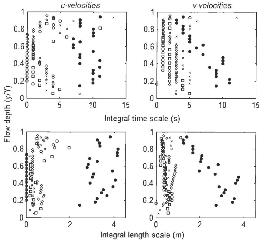
Figure 1.7: Integral time scales (ITS) and integral length scale (ILS) of open channel and ice covered flow conditions for the u and v components of the flow. p0 = \bullet ; p1 = \circ ; p2 = \square ; p3 = \diamond ; p4 = \times .
