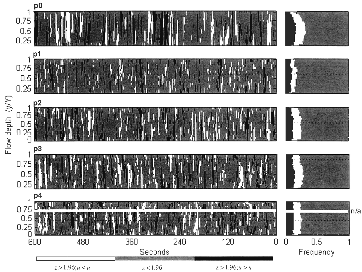
Figure 1.6: Clusters of coherent motions as revealed by the LISA algorithm when applied to the v component of the flow (refer to figure 1.5 for extended caption description).
