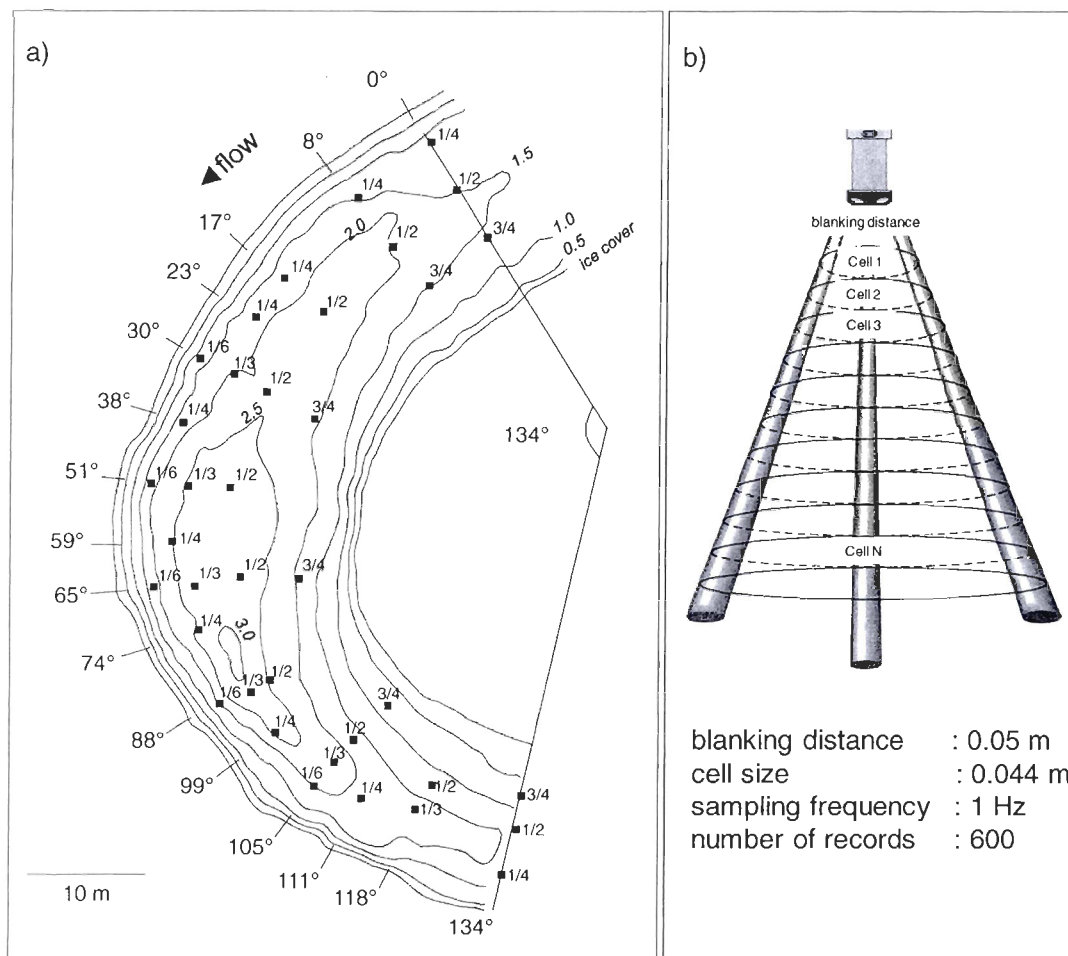
Figure 2.1 : a) Meander reach sampling scheme; b) PC-ADP sampling scheme.
