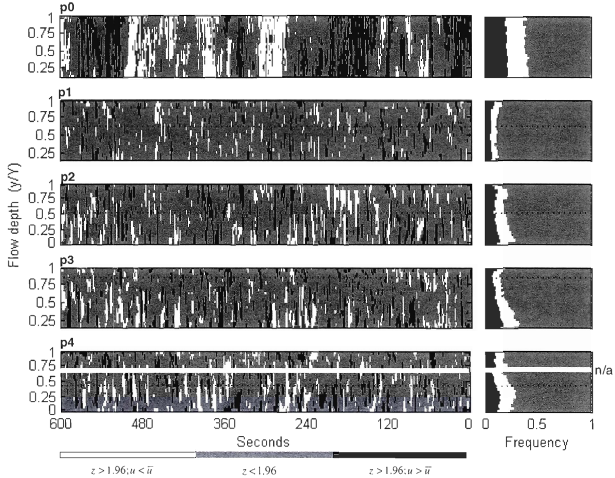
Figure 1.5: Clusters of coherent motions as revealed by the LISA algorithm when applied to the u component of the flow. Data with lower and higher than local average velocities are respectively presented as white and black cells. On the right hand of each profile, a frequency diagram illustrates how often cell velocities have been grouped in a given cluster type. The dot line is y_{uv=0}/Y .
