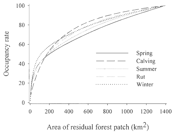
Figure 3. Relationships between the area of residual forest patch and the occupancy rate by caribou for each season, based on raw data.
