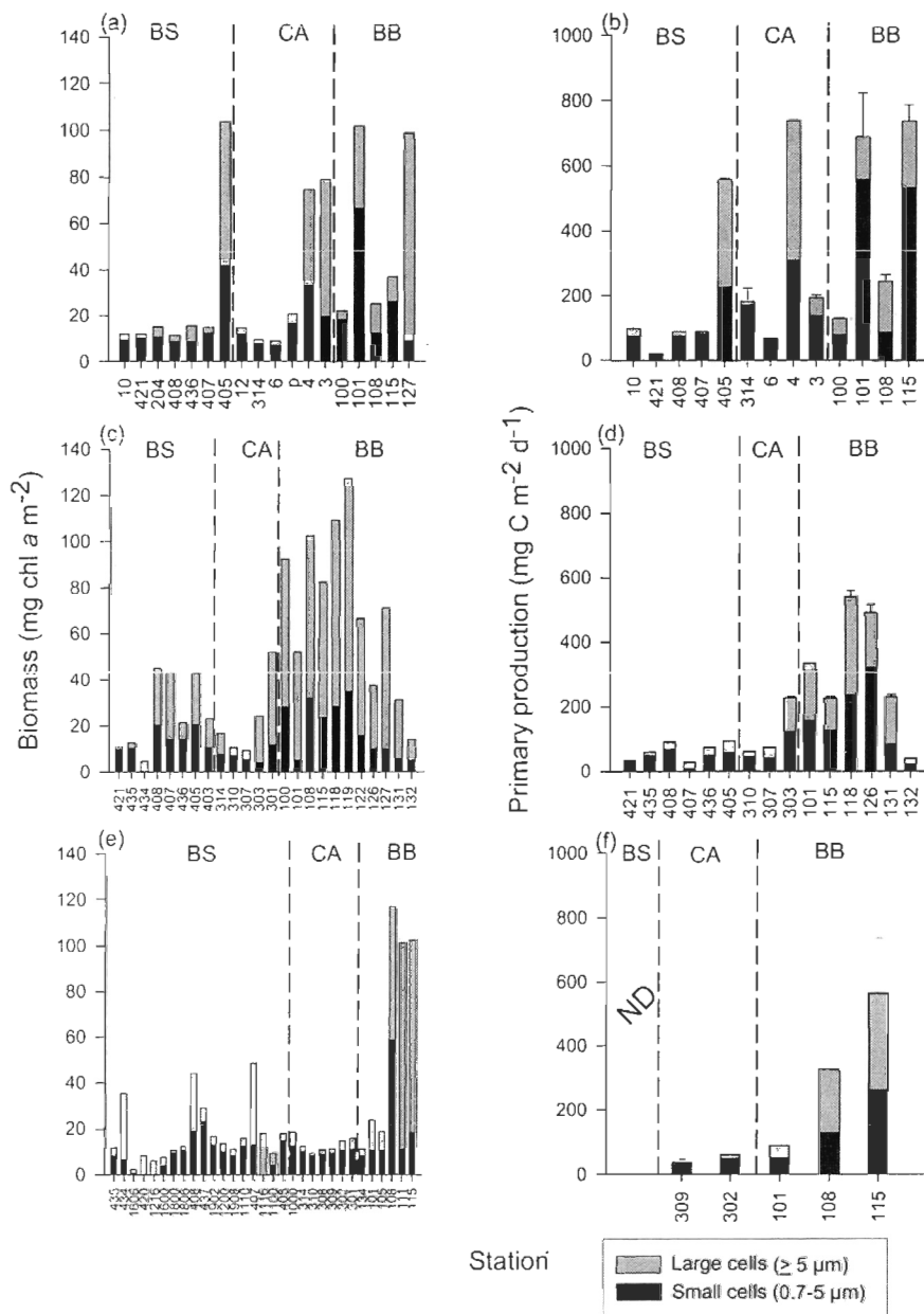
Fig. 3. Variations in phytoplankton (a, c, e) chlorophyll a (chl a ) biomass and (b, d, f) production for small (0.7 – 5 µm) and large (≥ 5 µm) cells integrated over the euphotic zone of stations across the Canadian High Arctic during (a, b) late summer 2005, (c, d) early fall 2006 and (e, f) fall 2007. In (b, d, f), vertical lines represent standard deviations of estimated rates. BS: Beaufort Sea; CA: Canadian Arctic Archipelago; BB: Baffin Bay; ND: no data available.
