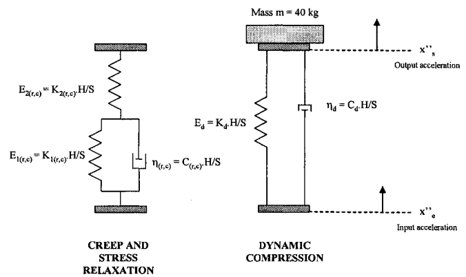
FIGURE 2 – Rheologic models of IVD using three elements ( E_{10} , E_{20} , \eta_0 ) for creep, three elements ( E_{1r} , E_{2r} , \eta_r ) for stress relaxation, and two elements ( E_d , \eta_d ) for dynamics; K_{10} , K_{1r} , K_{20} , K_{2r} and K_d are the stiffness of the associated springs; C_0 , C_r et C_d are the damping values; H et S are the disc height and cross-sectional area, respectively.
