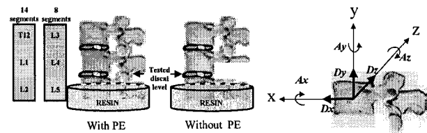
FIGURE 1 - Specimen preparation for the mobility tests with and without posterior elements (PE); reference axis located as followed: Ax, Ay, Az = frontal, axial, sagittal rotations; Dx, Dy, Dz = postero-anterior, vertical, transverse translations.
