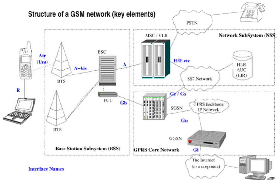
Figure 1.6 : architecture GSM
