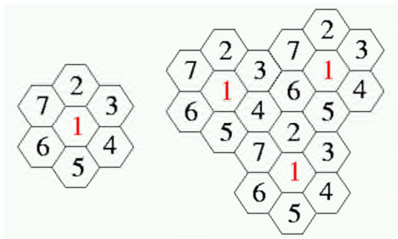
Figure 1.3 : concept cellulaire
