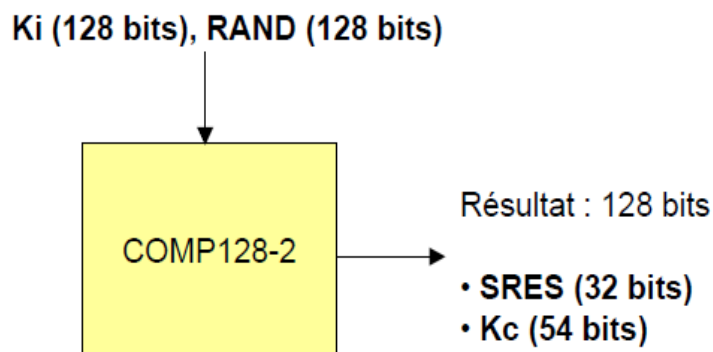
Figure I.7: Algorithme COMP128-2
