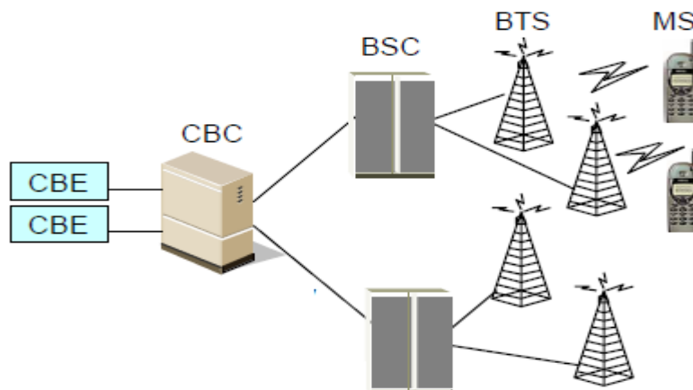
Figure I.12: Architecture du service SMS Cell Broadcast
