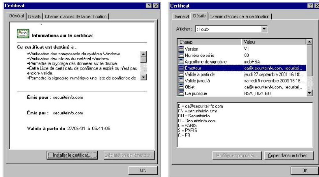
Figure II.8: Exemple d'un Certificat X509
