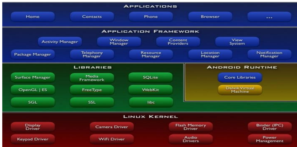
Figure III.8: Anatomie d'Android
