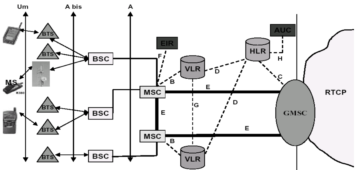
Figure I.2 : interfaces GSM
