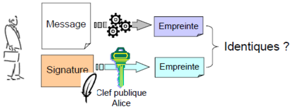
Figure II.6: vérification de signature
