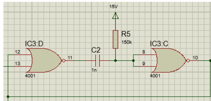
Figure 2.14: Circuit du monostable
