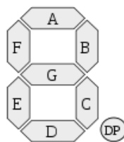
Figure 2.33: Afficheur 7 segments
