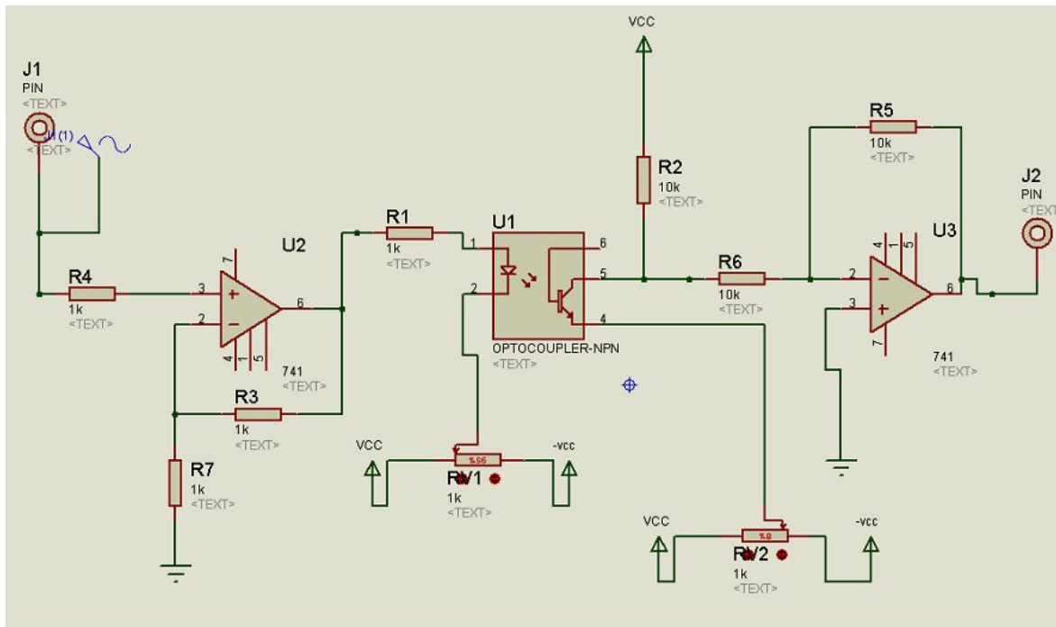
Figure II.10 : circuit Opto-isolateur
