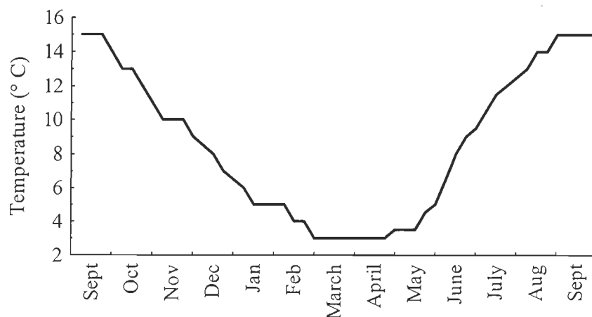
Figure III. 1 : Annual temperature profile of freshwater at the Station aquicole of ISMER/UQAR at Rimouski (Qc, Canada).
