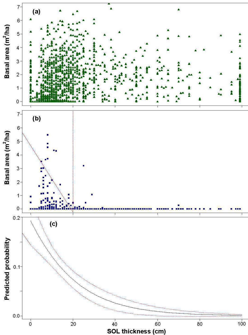
Fig. 1.4 Basal area ( \text{m}^2/\text{ha} ) of black spruce (A) and aspen (B) in PSPs plotted against SOL thickness (cm). Distribution of aspen seems to be limited by a threshold (dashed line) of \sim 20 cm. Predicted probability to find aspen along the SOL thickness gradient in the PSPs (C) with the confidence interval at 95% (dotted lines) determined through logistic regression.
